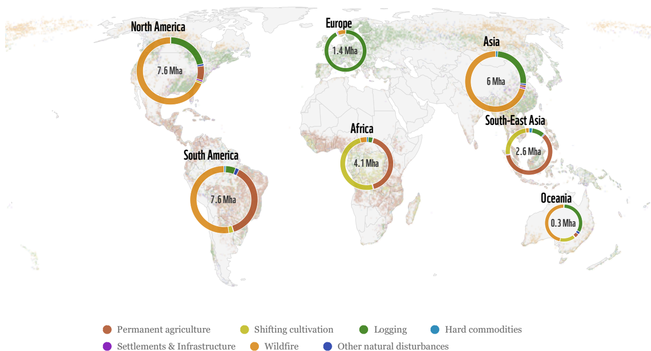
Figure 2. Tree cover loss in 2024 ( Global Forest Change v1.12 ), disaggregated by driver following Sims et al. (2025)
