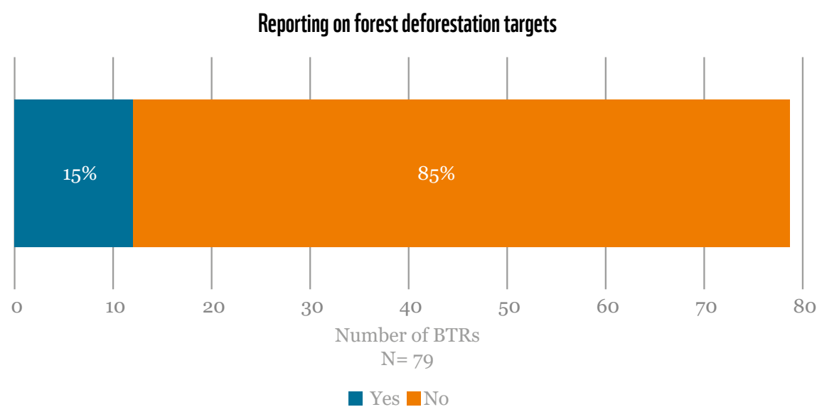
Figure 4. Reporting on deforestation targets in BTRs
