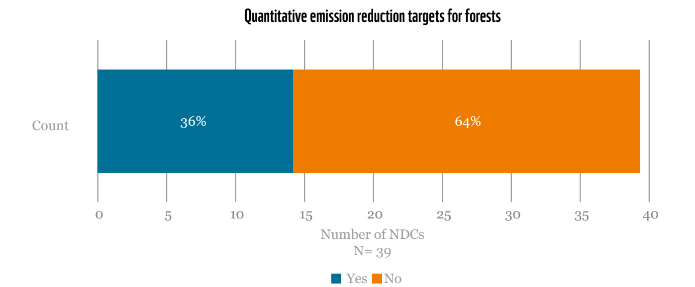
Figure 10. Quantitative emission reduction targets for forests in NDCs
