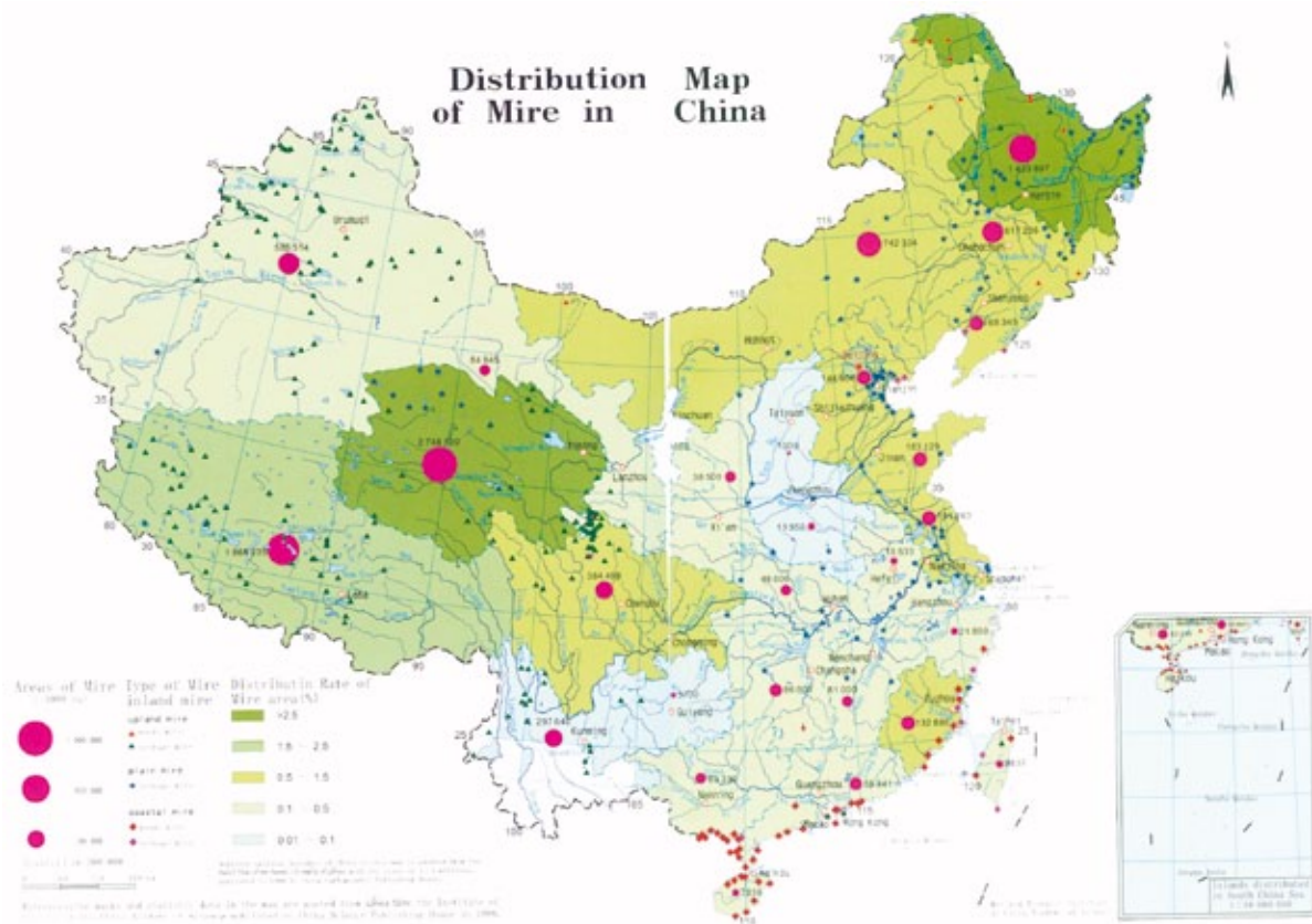
Figure 15: Distribution of “mires” in China (from State Forestry Administration P.R. China, 2002)
