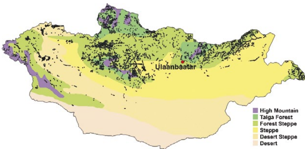
Figure 17: Peatland distribution in Mongolia (from Minayeva et al. , 2004)
